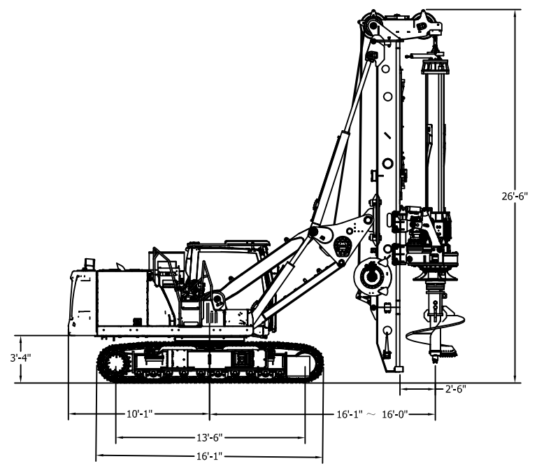
TRANSPORT WEIGHT WITH KELLY BAR 99,000 LBS TRANSPORT WEIGHT W/O KELLY BAR 92,400 LBS
