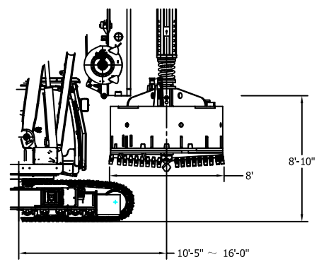
TOOL CLEARANCE W/O MAST FOOT AND SHORT KELLY BAR
