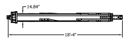
4 - ELEMENT LOCKING BAR TRANSPORT WEIGHT 6,600 LBS
