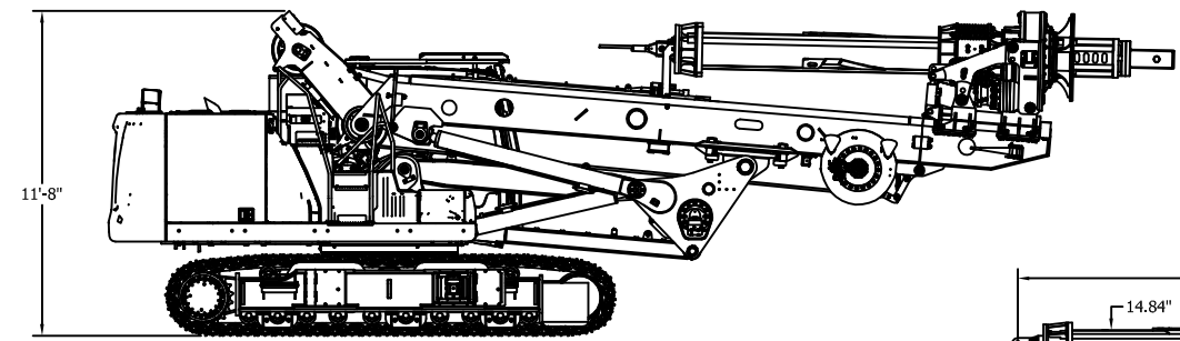
TRANSPORT WEIGHT WITH KELLY BAR 99,000 LBS TRANSPORT WEIGHT W/O KELLY BAR 92,400 LBS
