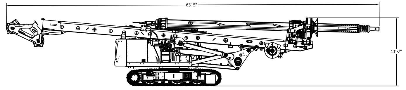
TRANSPORT WEIGHT 109,000 LBS WITH KELLY BAR TRANSPORT WEIGHT 95,800 LBS W/O KELLY BAR
